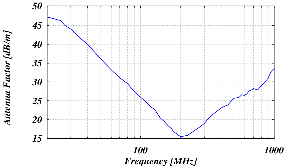
Antenna Factor
